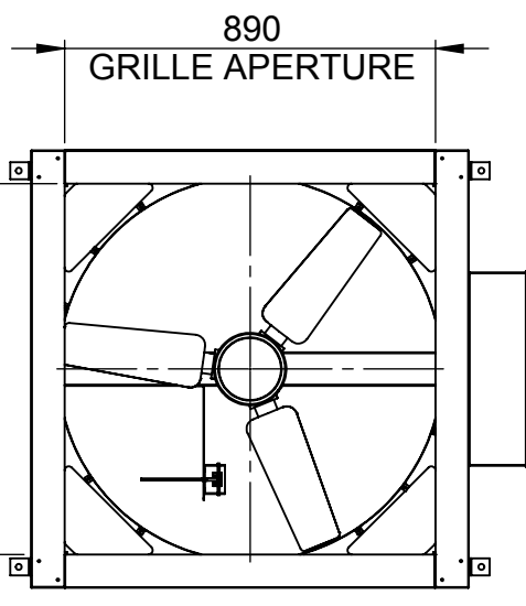
UNDERSIDE VIEW
