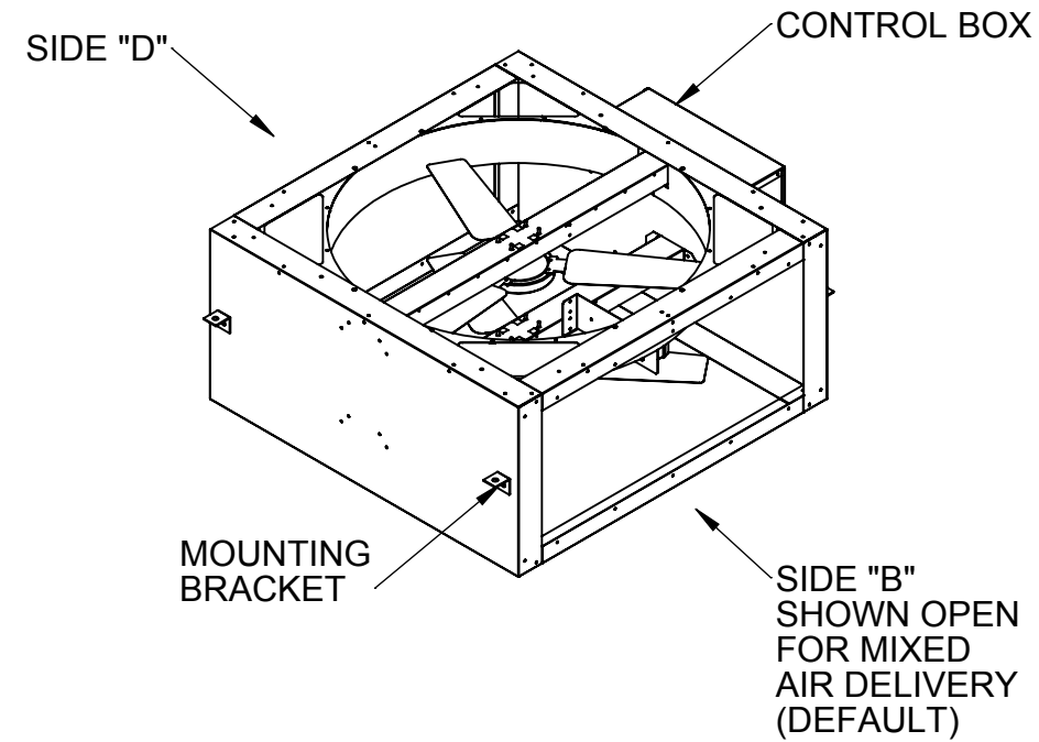
ISOMETRIC
