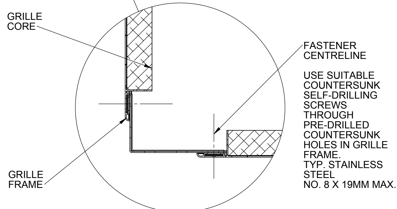
DETAIL A SCALE 1 : 2 GRILLE FIXINGS
