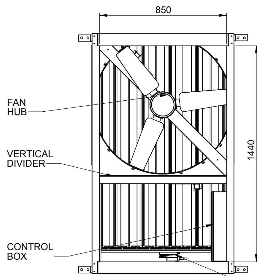
UNDERSIDE VIEW
