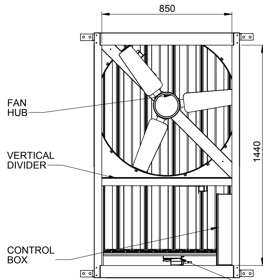
UNDERSIDE VIEW
