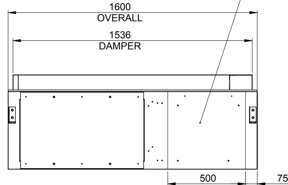
"A" SIDE (SHOWN WITH MIXED AIR DELIVERY CLOSED)
