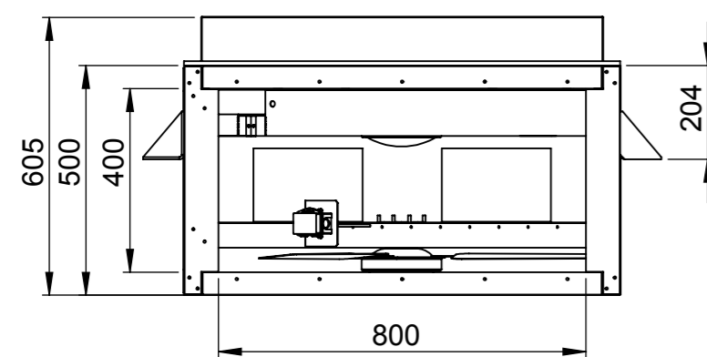
"B" SIDE (SHOWN WITH MIXED AIR DELIVERY OPEN)
