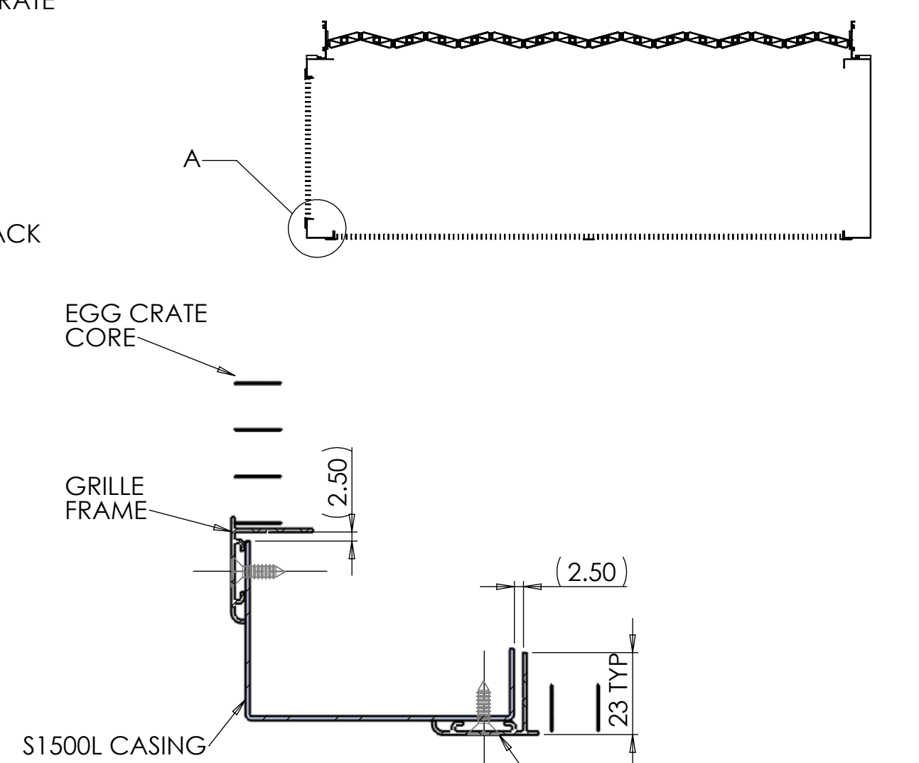
DETAIL A SCALE 2 : 3
